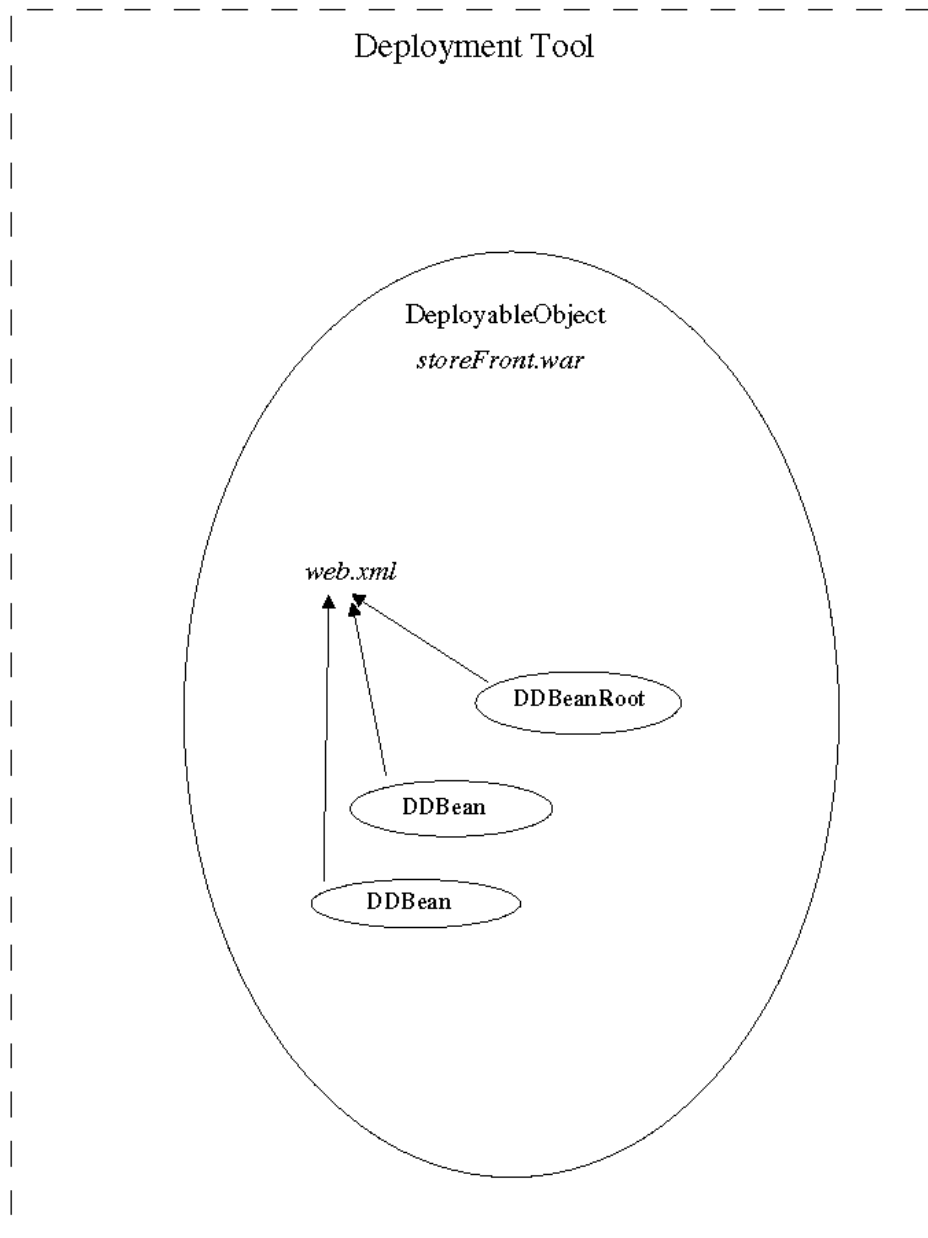
Figure 3.2 J2EE Standalone Module
